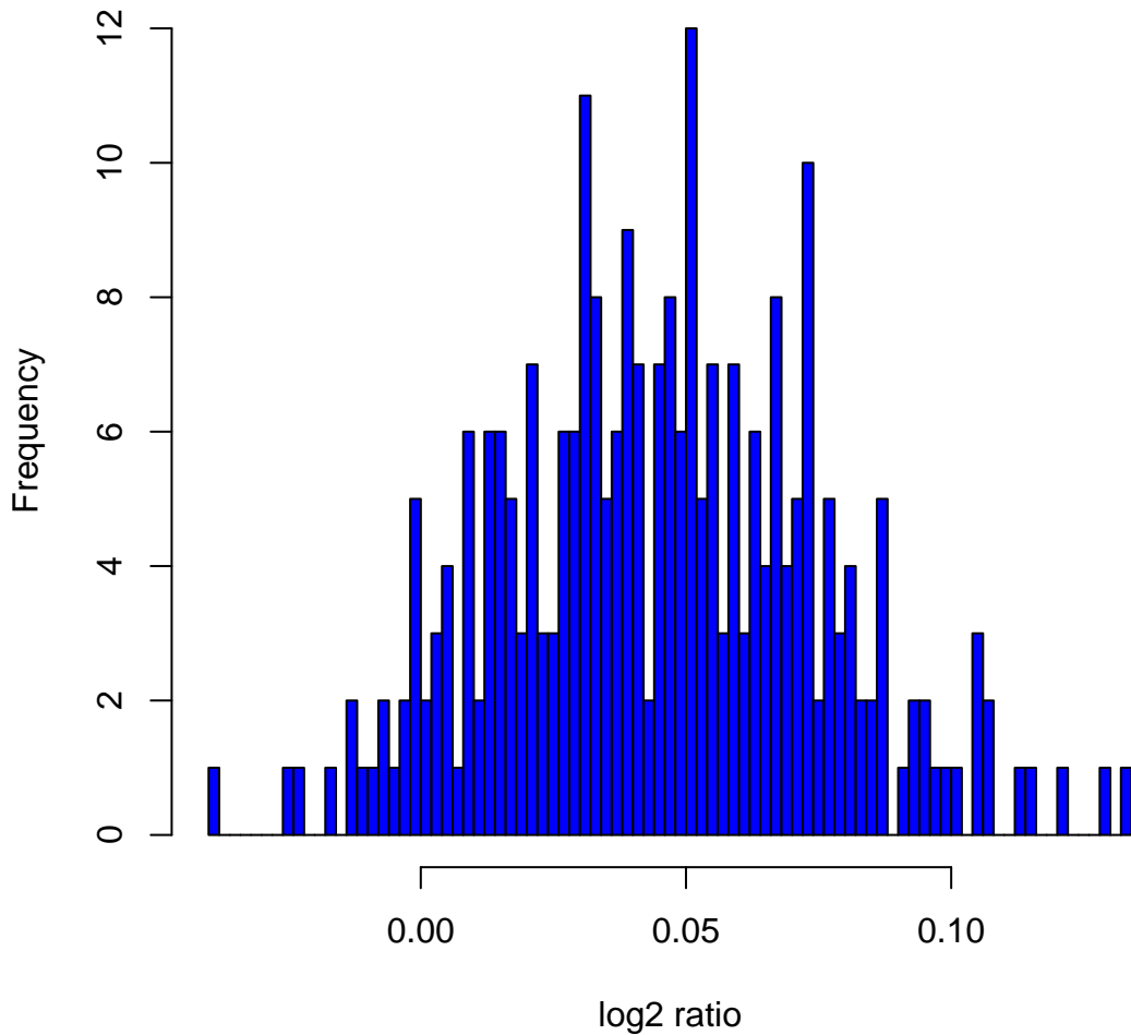
Histogram of log2ratios in 270 HapMap samples at clone Chr2tp-24H12
