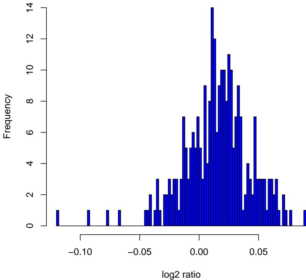
Histogram of log2ratios in 270 HapMap samples at clone Chr2tp-25C10
