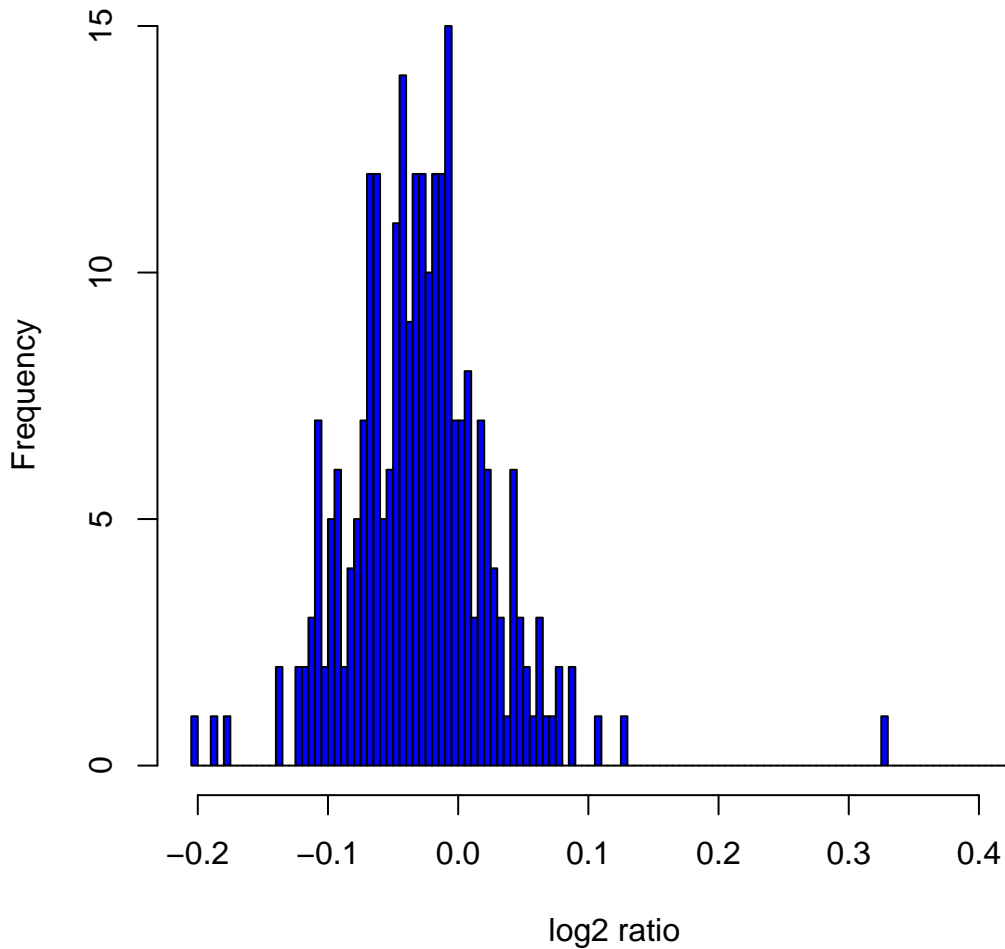
Histogram of log2ratios in 270 HapMap samples at clone Chr2tp-25D10
