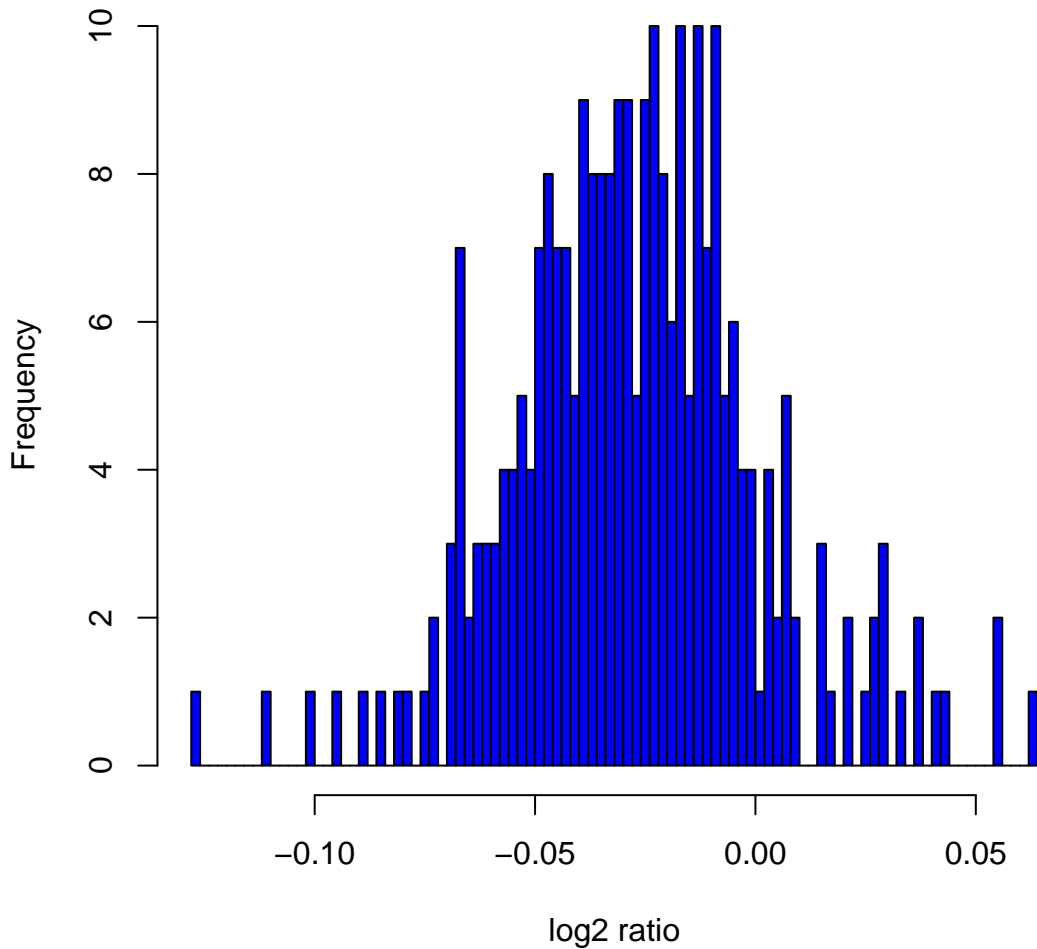
Histogram of \log_2 ratios in 270 HapMap samples at clone Chr2tp-25G10
