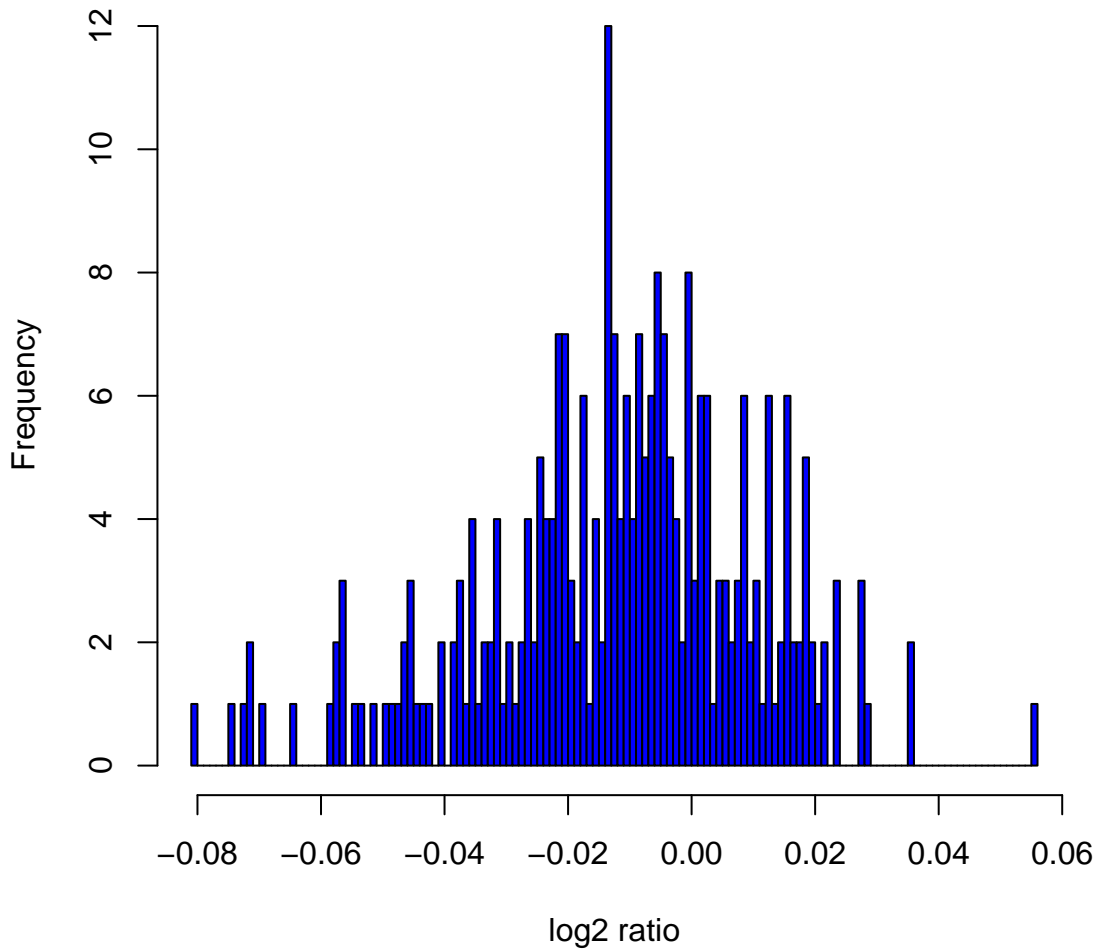
Histogram of \log_2 ratios in 270 HapMap samples at clone Chr2tp-26A6
