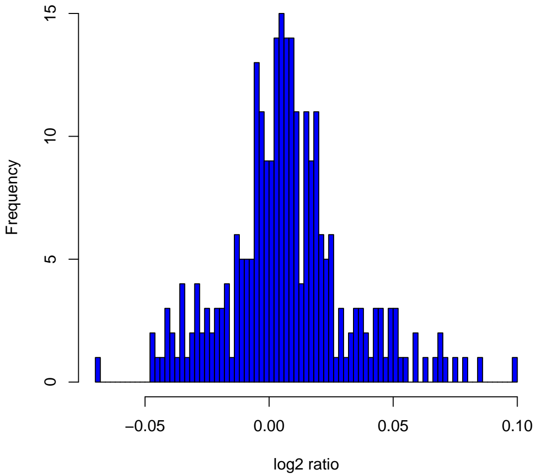
Histogram of log 2 ratios in 270 HapMap samples at clone Chr2tp-26B2
