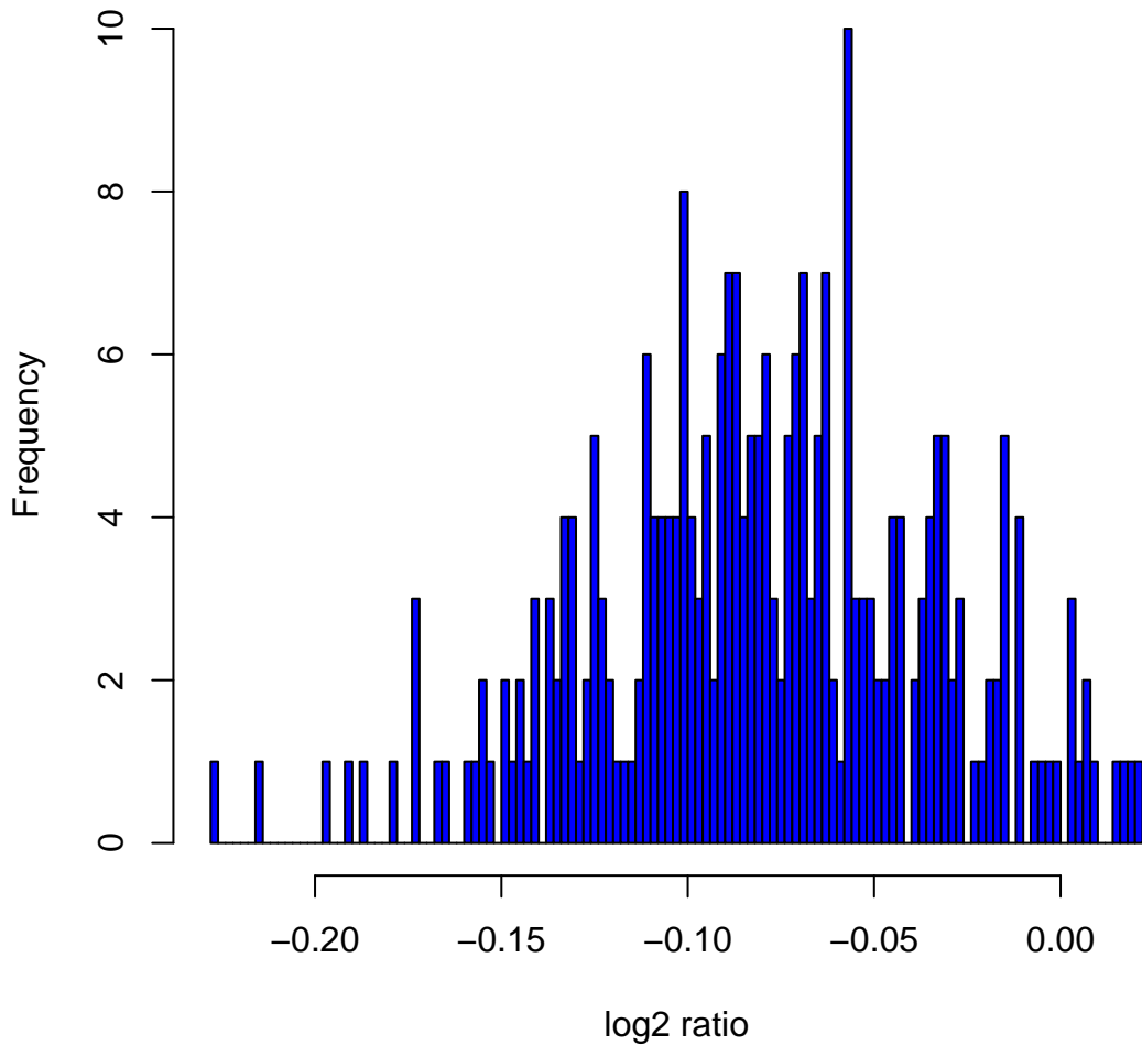
Histogram of log 2 ratios in 270 HapMap samples at clone Chr2tp-26C2
