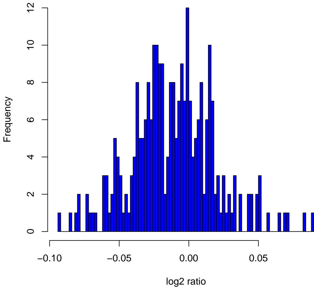
Histogram of log 2 ratios in 270 HapMap samples at clone Chr2tp-26C7
