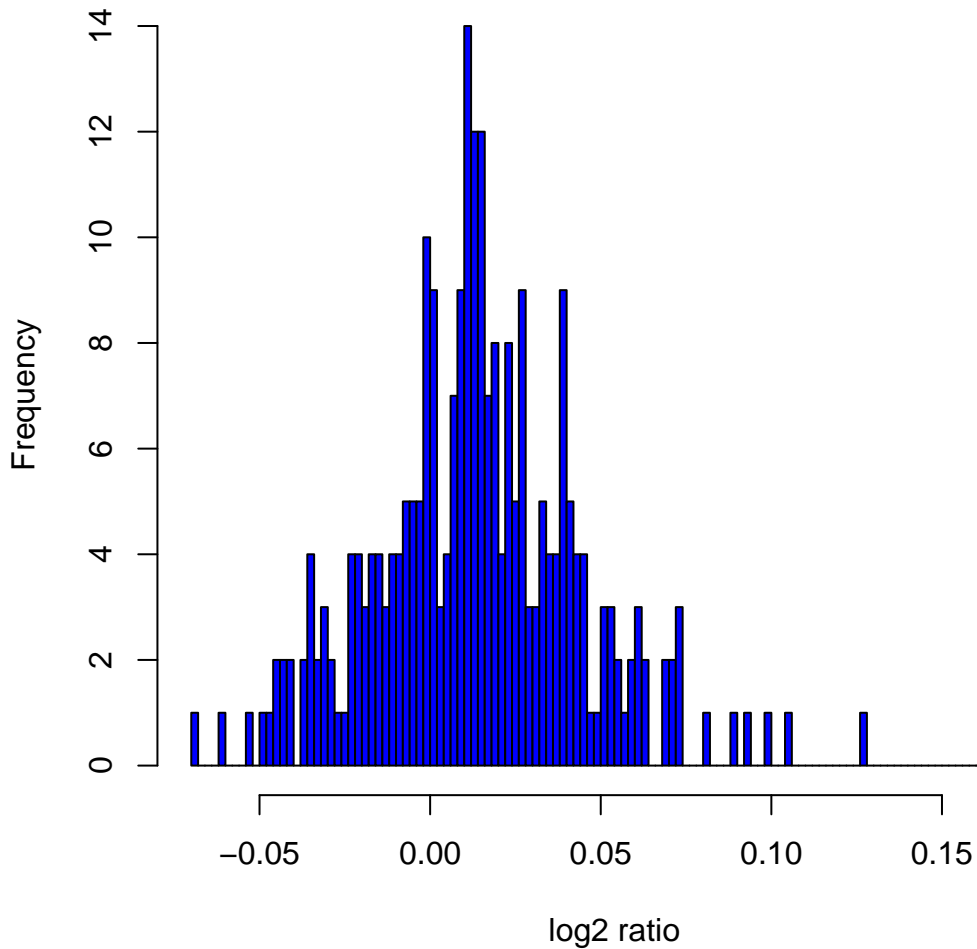
Histogram of \log_2 ratios in 270 HapMap samples at clone Chr2tp-26D3
