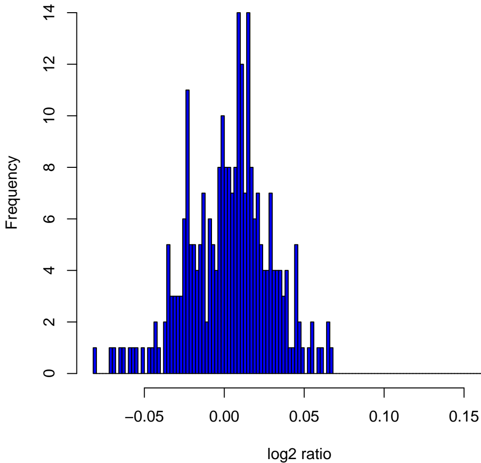
Histogram of \log_2 ratios in 270 HapMap samples at clone Chr2tp-28C9
