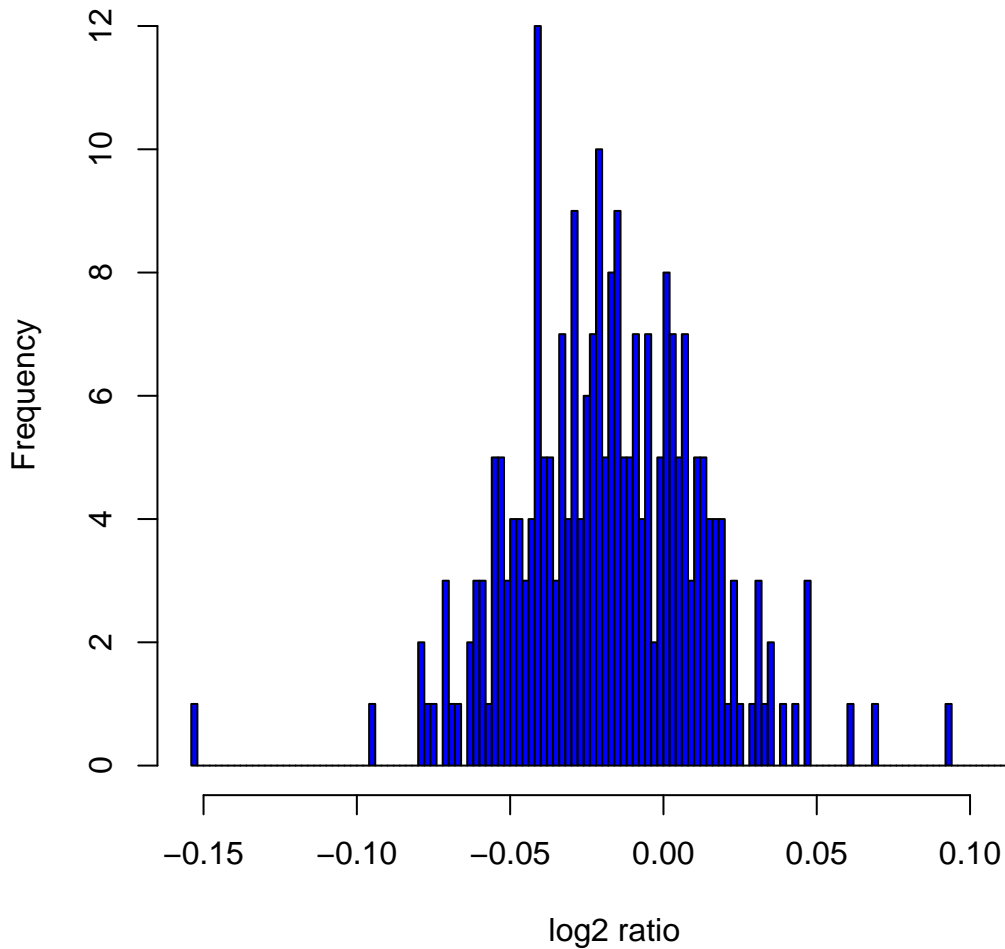
Histogram of log 2 ratios in 270 HapMap samples at clone Chr2tp-28H1
