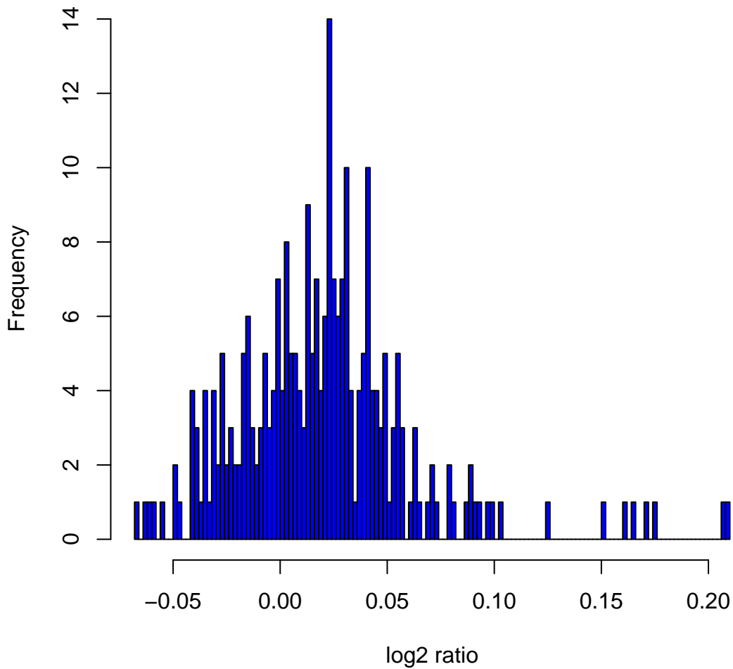
Histogram of log 2 ratios in 270 HapMap samples at clone Chr2tp-28H8
