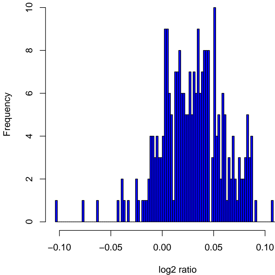
Histogram of log2ratios in 270 HapMap samples at clone Chr2tp-29B12
