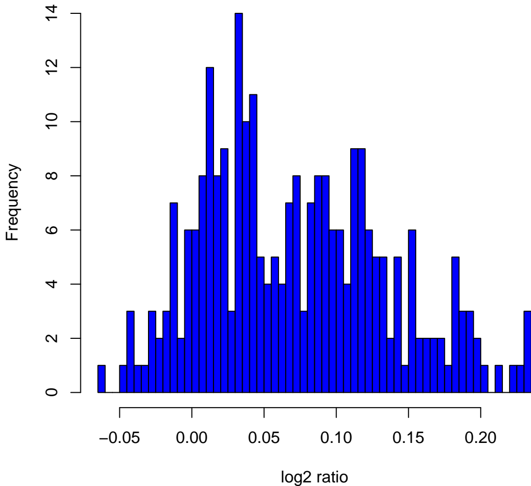
Histogram of log2ratios in 270 HapMap samples at clone Chr2tp-29C12
