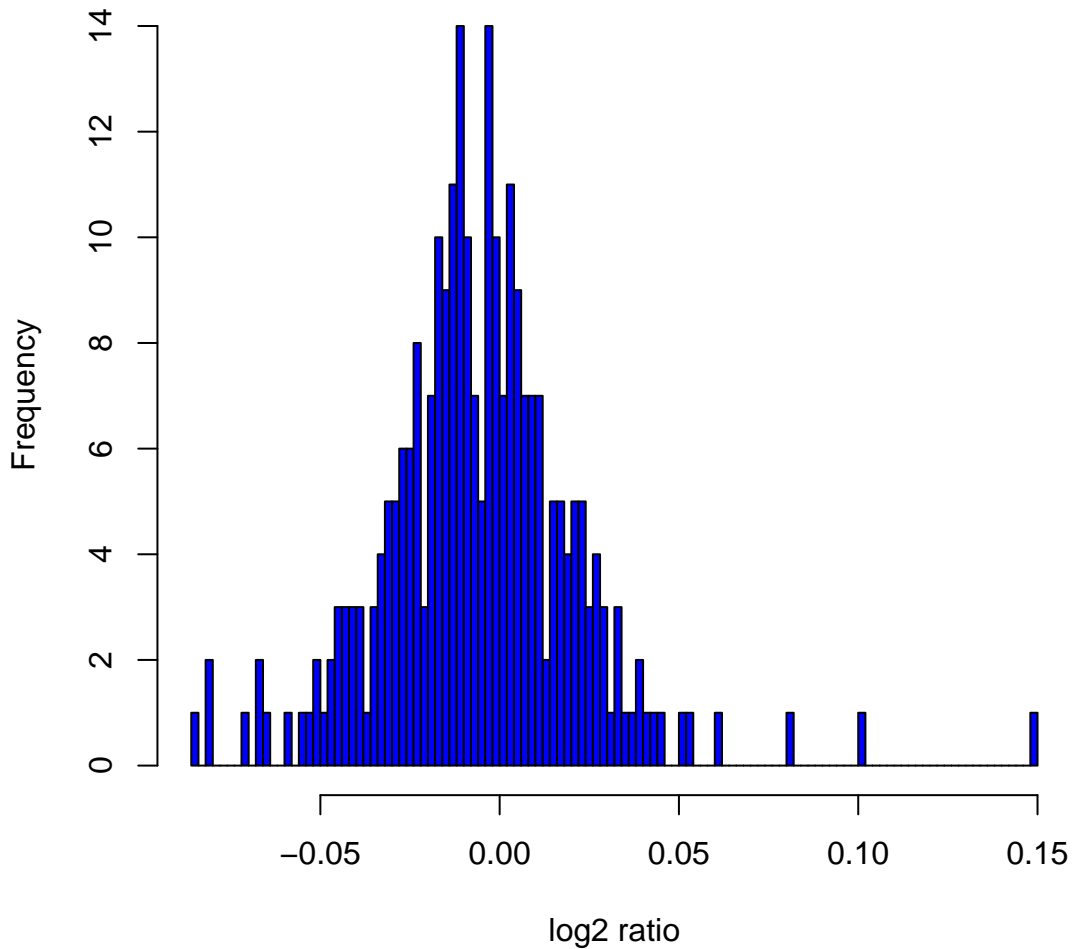
Histogram of \log_2 ratios in 270 HapMap samples at clone Chr2tp-29D5
