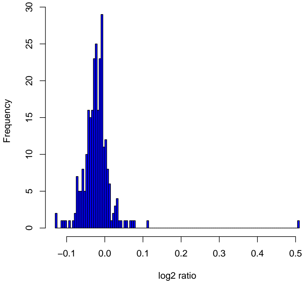
Histogram of log2ratios in 270 HapMap samples at clone Chr2tp-29F3
