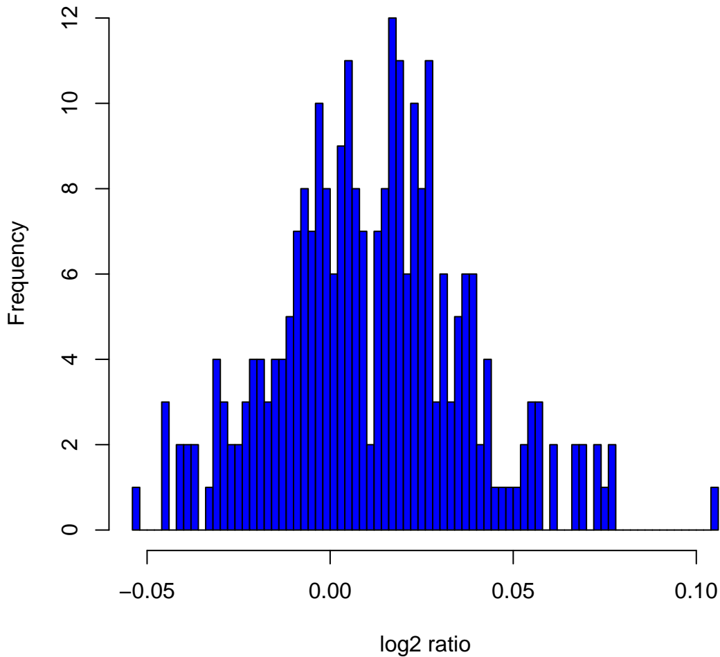
Histogram of log2ratios in 270 HapMap samples at clone Chr2tp-29G10
