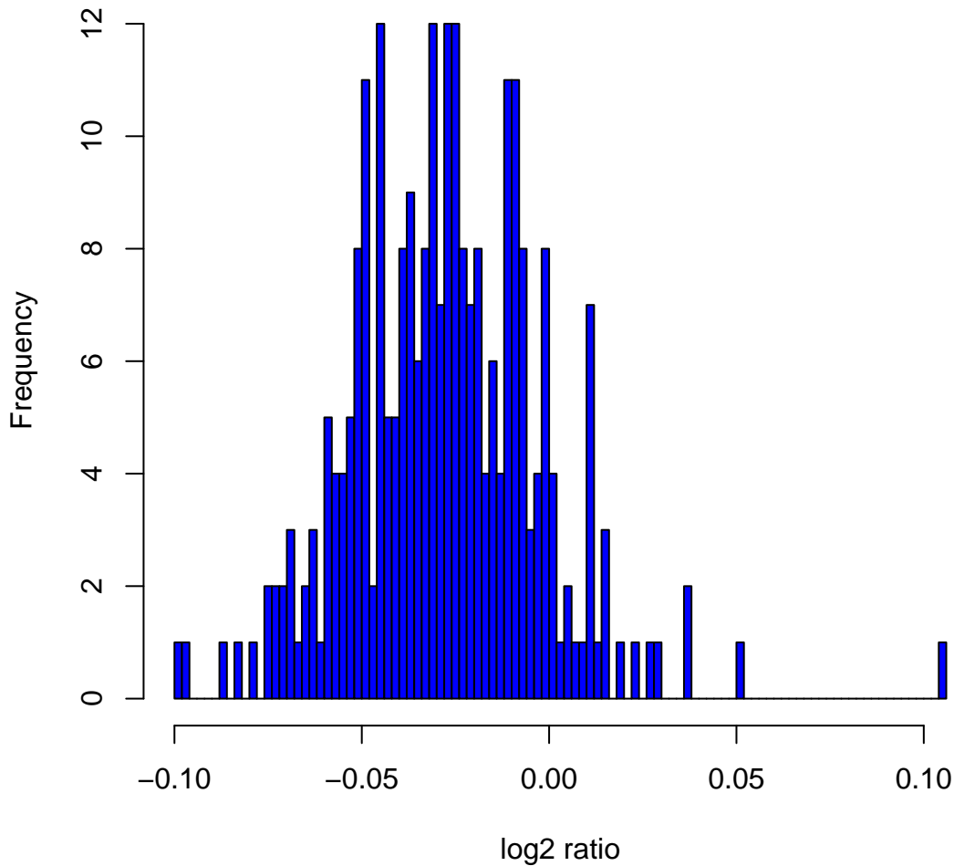
Histogram of log 2 ratios in 270 HapMap samples at clone Chr2tp-2D11
