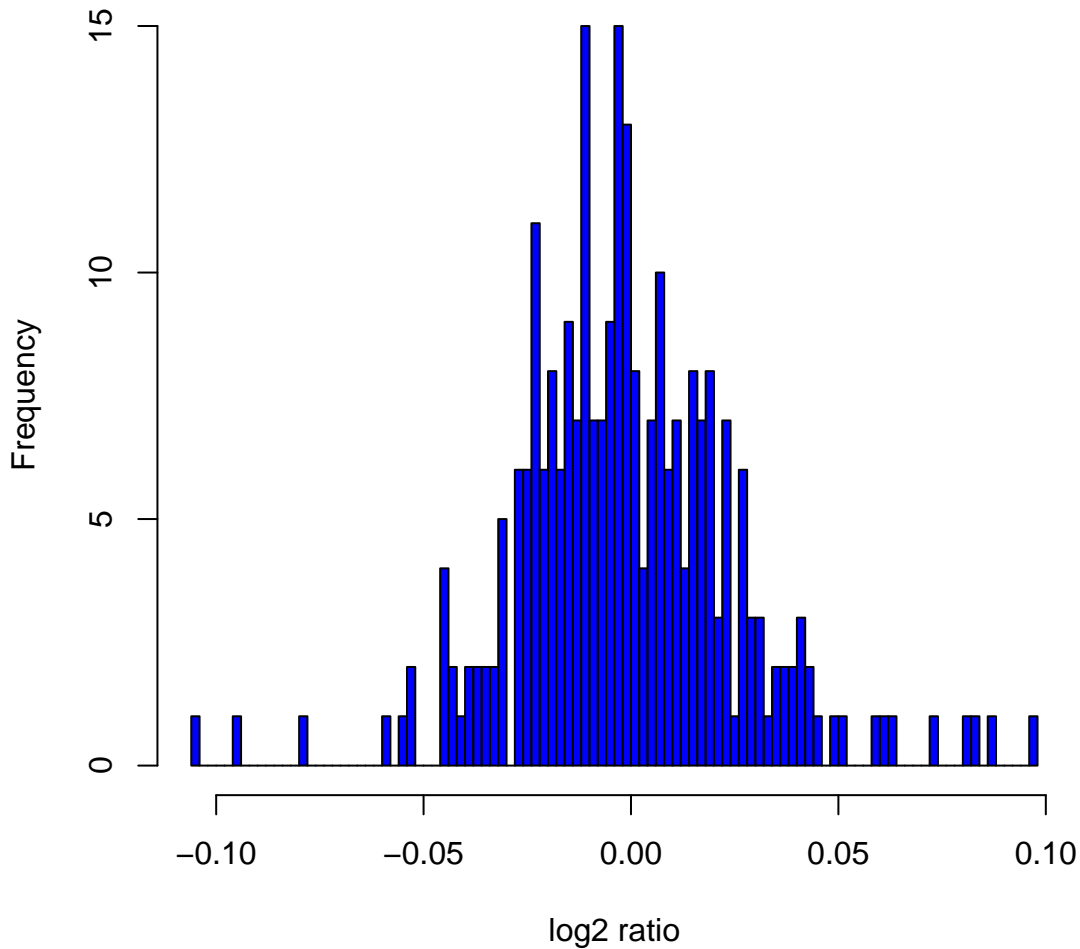
Histogram of \log_2 ratios in 270 HapMap samples at clone Chr2tp-2D4
