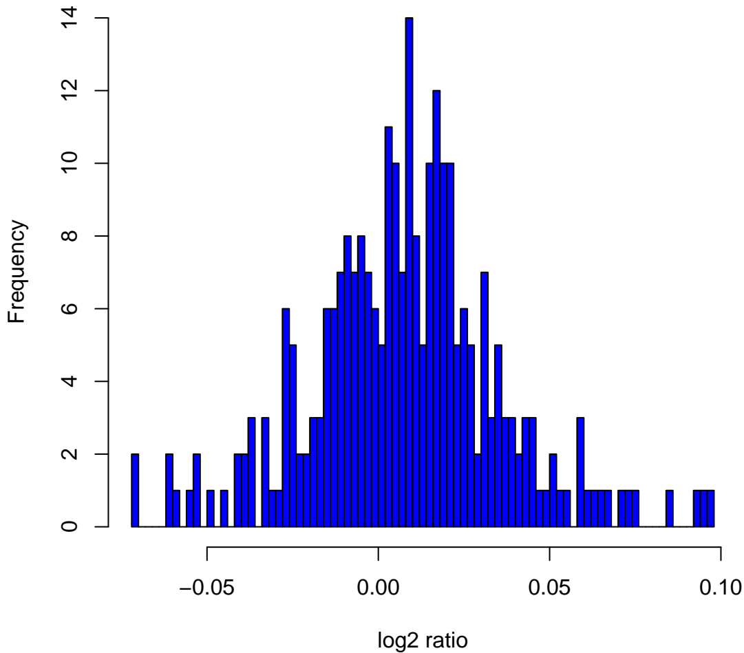
Histogram of log 2 ratios in 270 HapMap samples at clone Chr2tp-2E4
