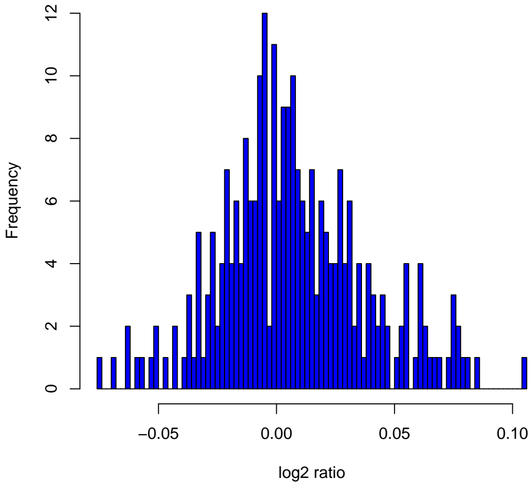
Histogram of \log_2 ratios in 270 HapMap samples at clone Chr2tp-2H9
