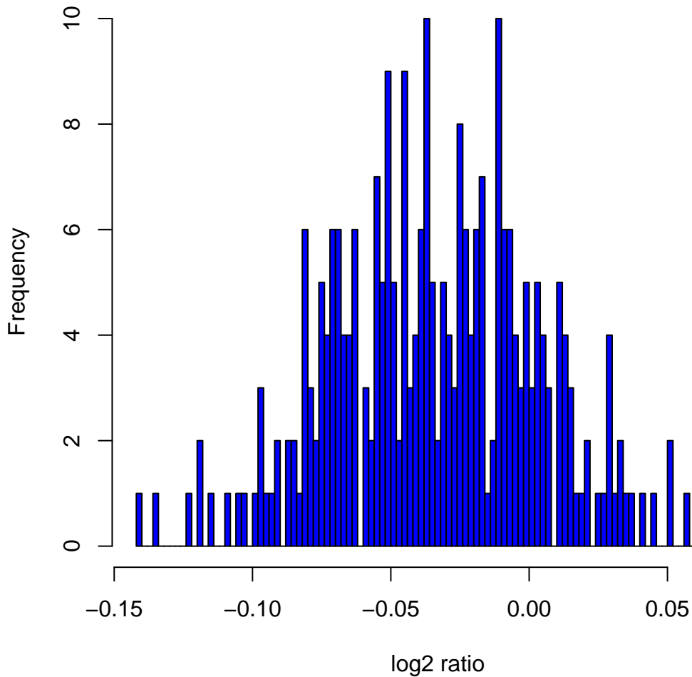
Histogram of log2ratios in 270 HapMap samples at clone Chr2tp-30A11
