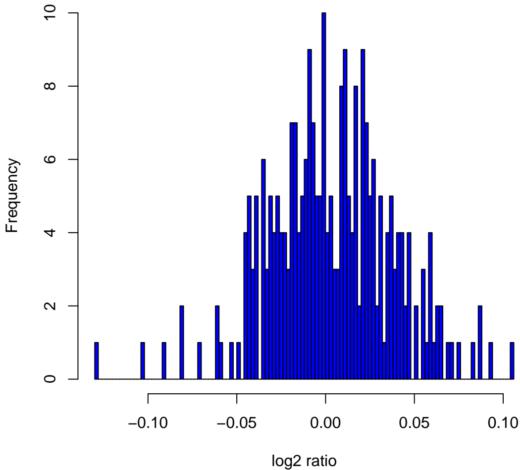
Histogram of log2ratios in 270 HapMap samples at clone Chr2tp-30B12
