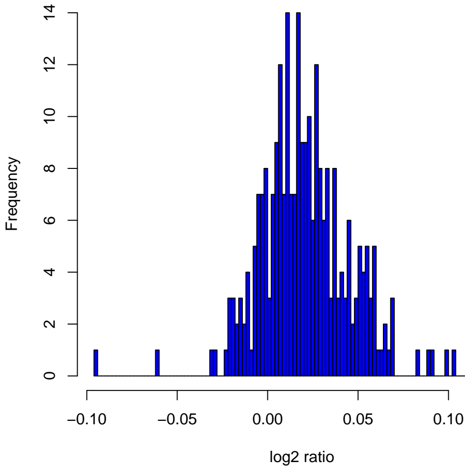
Histogram of log2ratios in 270 HapMap samples at clone Chr2tp-30C4
