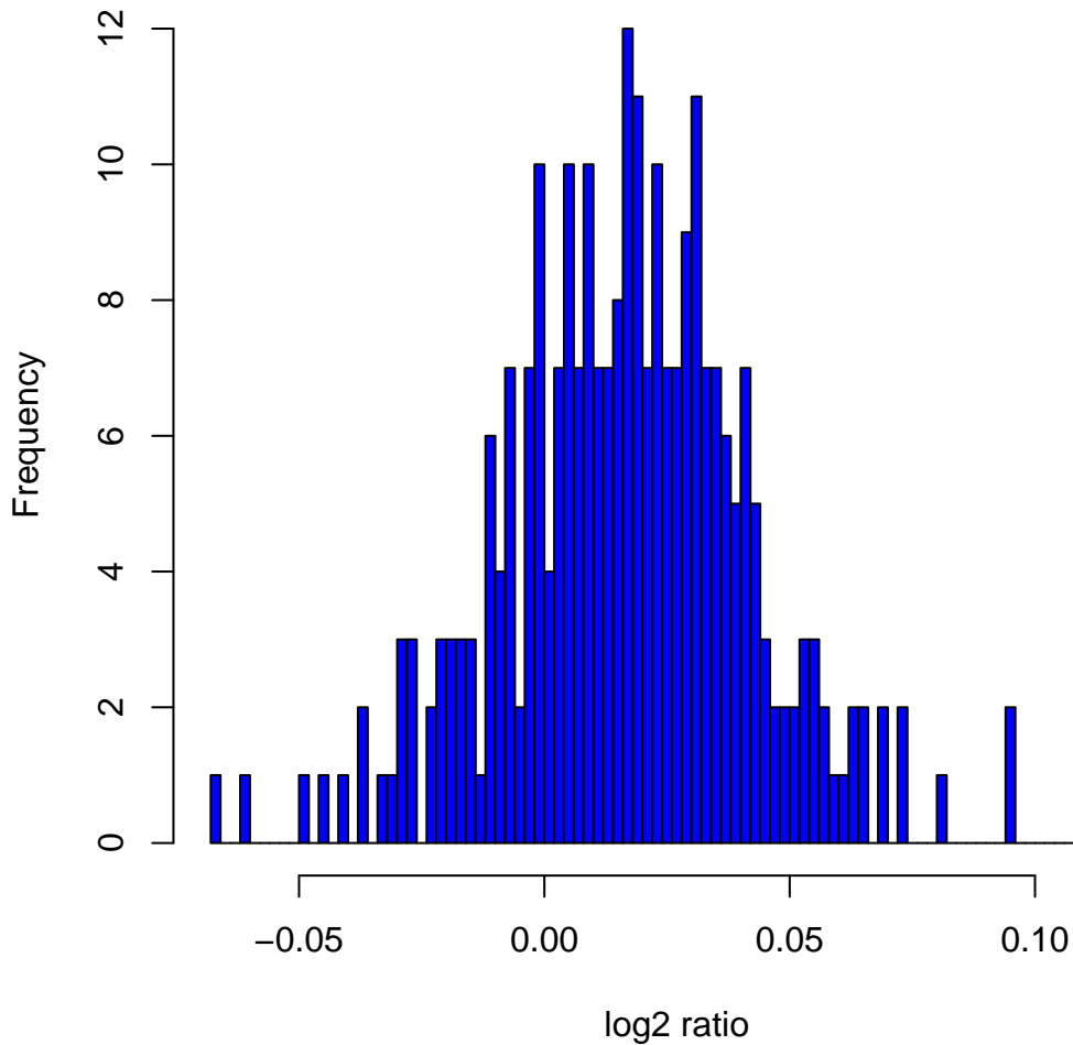
Histogram of log2ratios in 270 HapMap samples at clone Chr2tp-30G11
