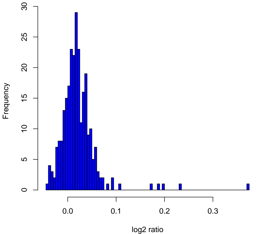
Histogram of log2ratios in 270 HapMap samples at clone Chr2tp-30G12
