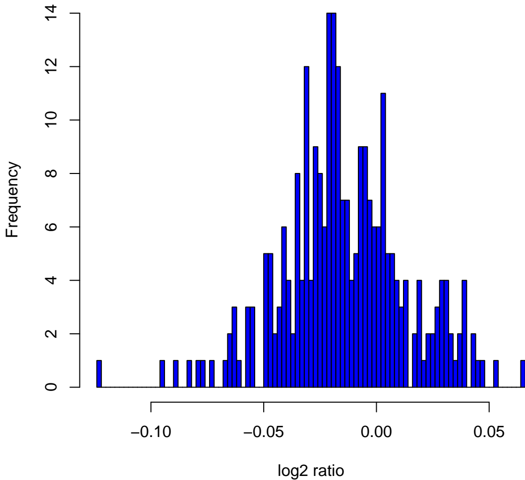
Histogram of log 2 ratios in 270 HapMap samples at clone Chr2tp-30G6
