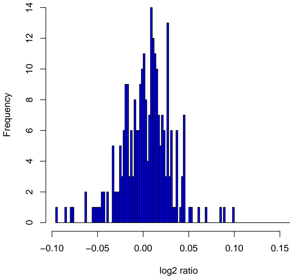
Histogram of log 2 ratios in 270 HapMap samples at clone Chr2tp-30H7
