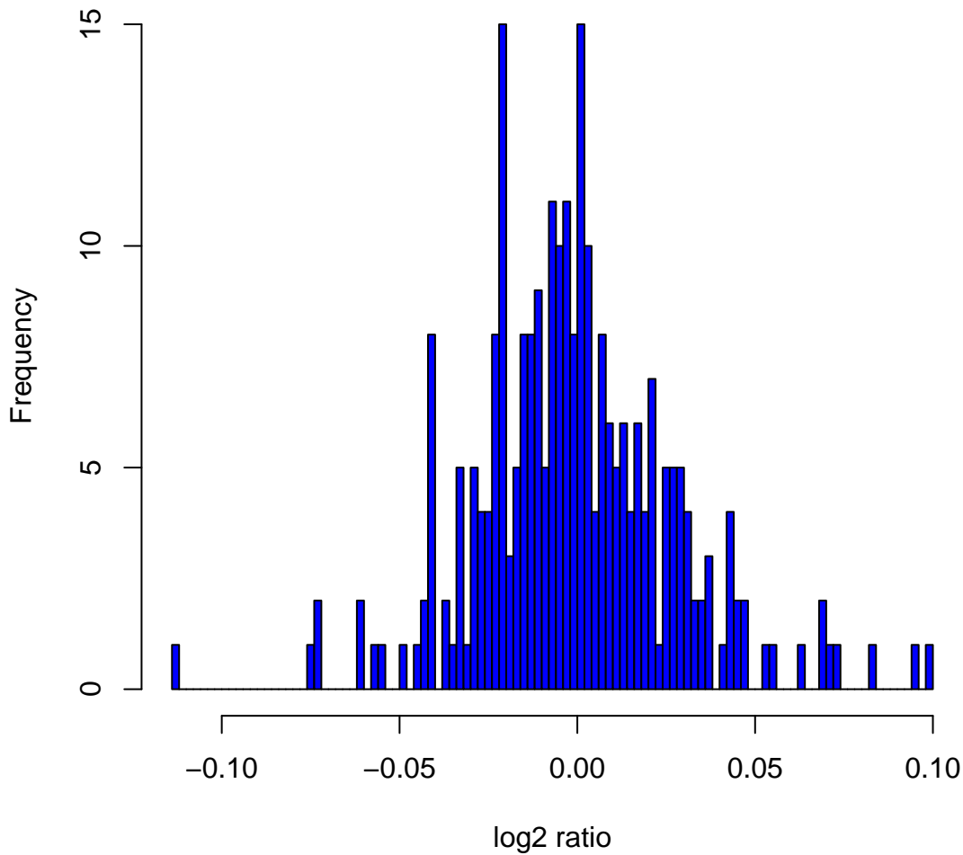
Histogram of log2ratios in 270 HapMap samples at clone Chr2tp-31A7
