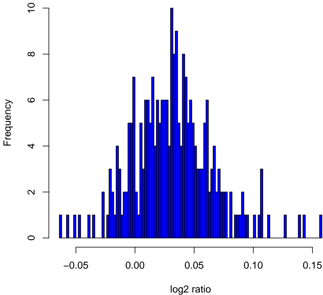
Histogram of log 2 ratios in 270 HapMap samples at clone Chr2tp-31C2
