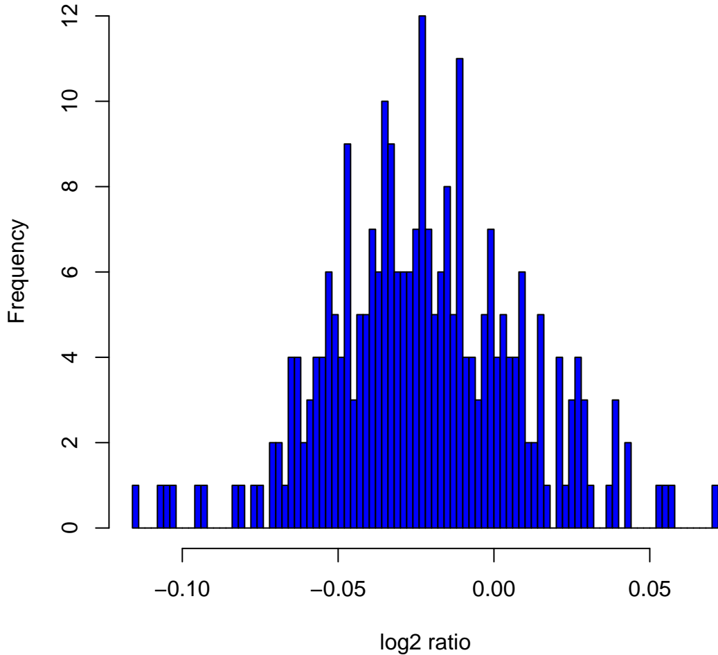
Histogram of log 2 ratios in 270 HapMap samples at clone Chr2tp-31D5
