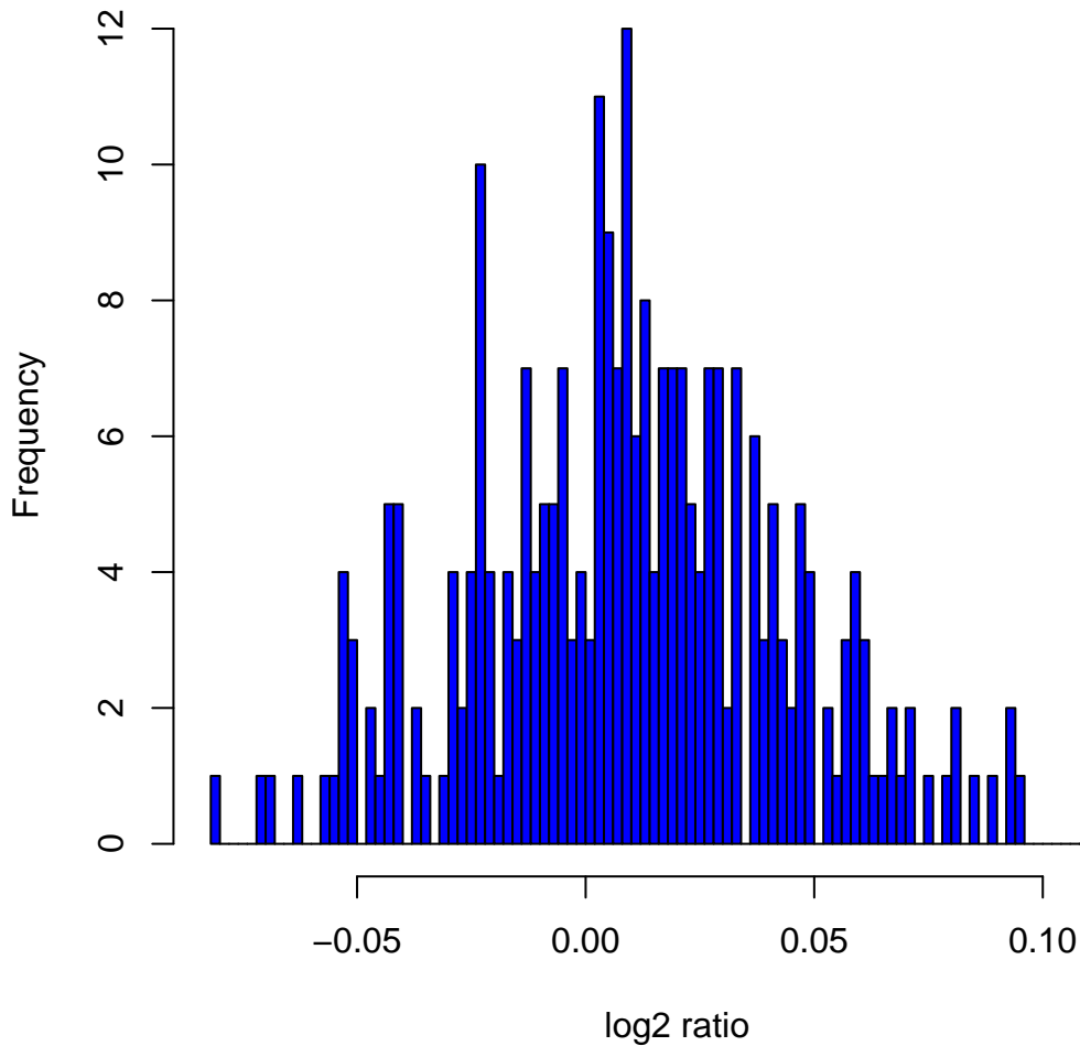
Histogram of log 2 ratios in 270 HapMap samples at clone Chr2tp-31E9
