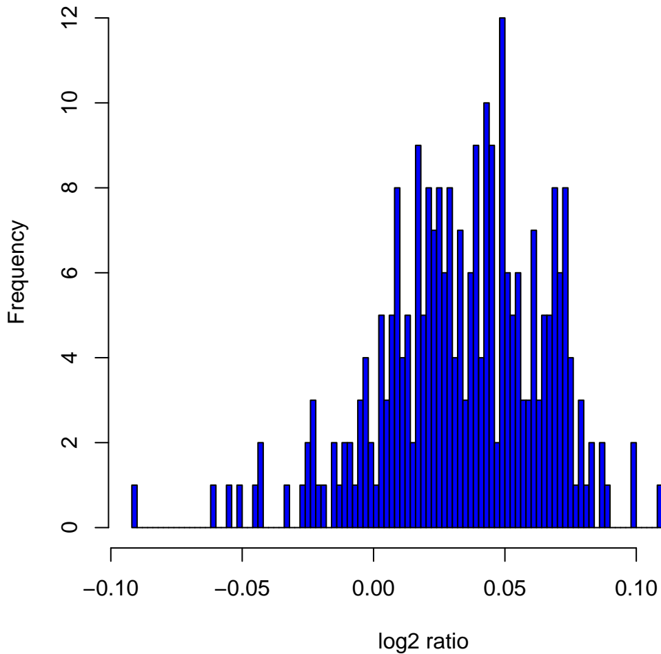
Histogram of log 2 ratios in 270 HapMap samples at clone Chr2tp-3A4
