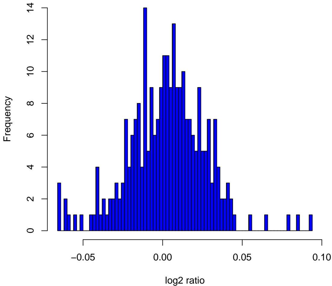
Histogram of \log_2 ratios in 270 HapMap samples at clone Chr2tp-3A5
