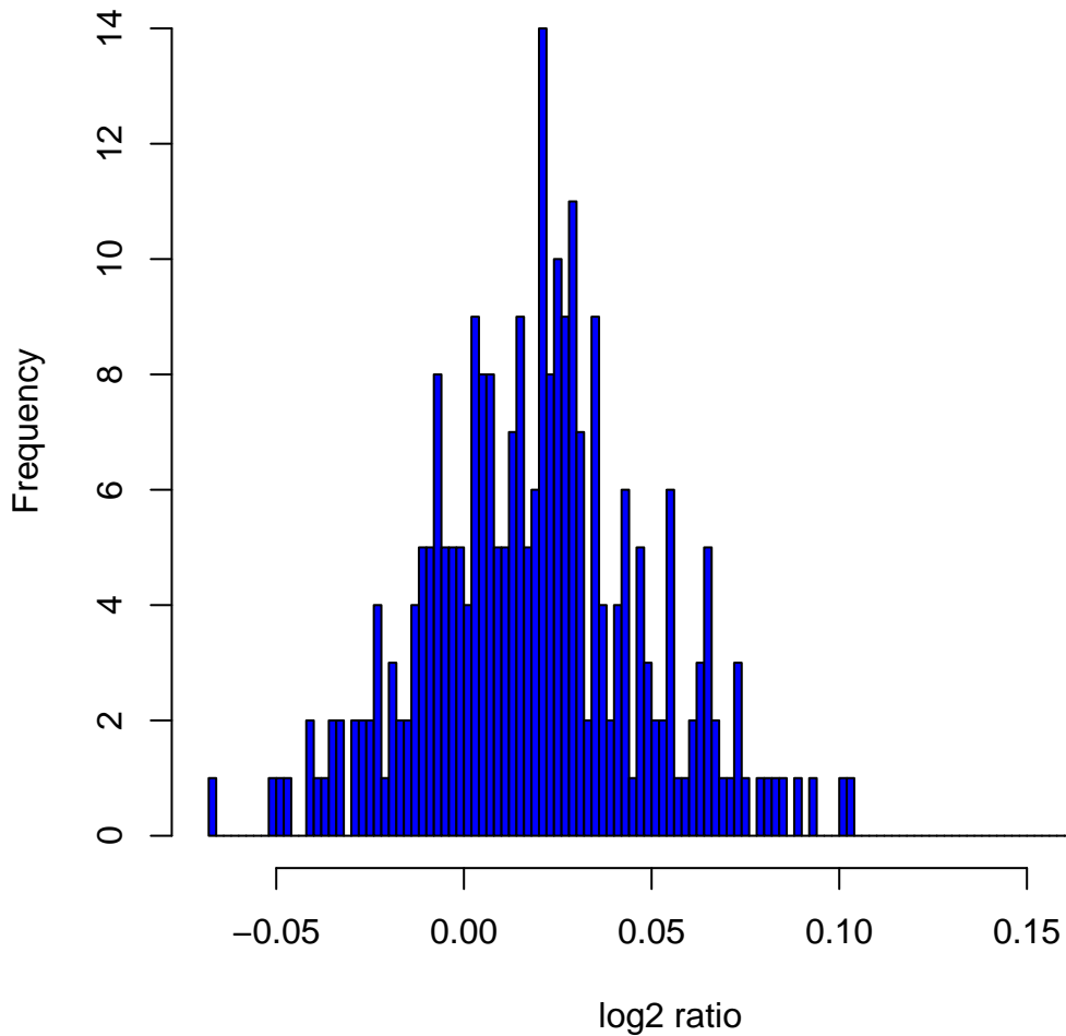
Histogram of \log_2 ratios in 270 HapMap samples at clone Chr2tp-3C9
