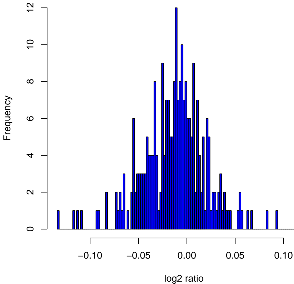
Histogram of log 2 ratios in 270 HapMap samples at clone Chr2tp-3F4
