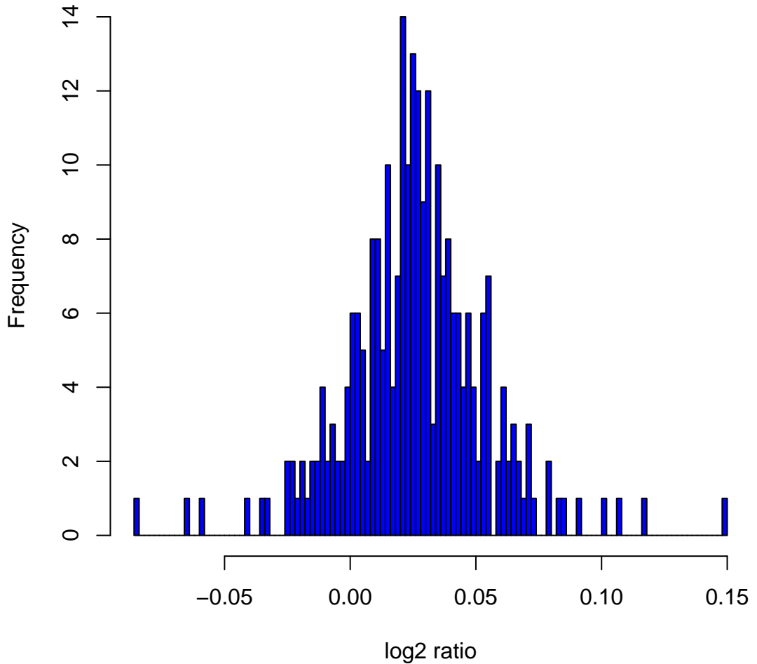
Histogram of log 2 ratios in 270 HapMap samples at clone Chr2tp-3G11
