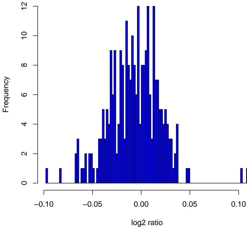
Histogram of log 2 ratios in 270 HapMap samples at clone Chr2tp-4A11
