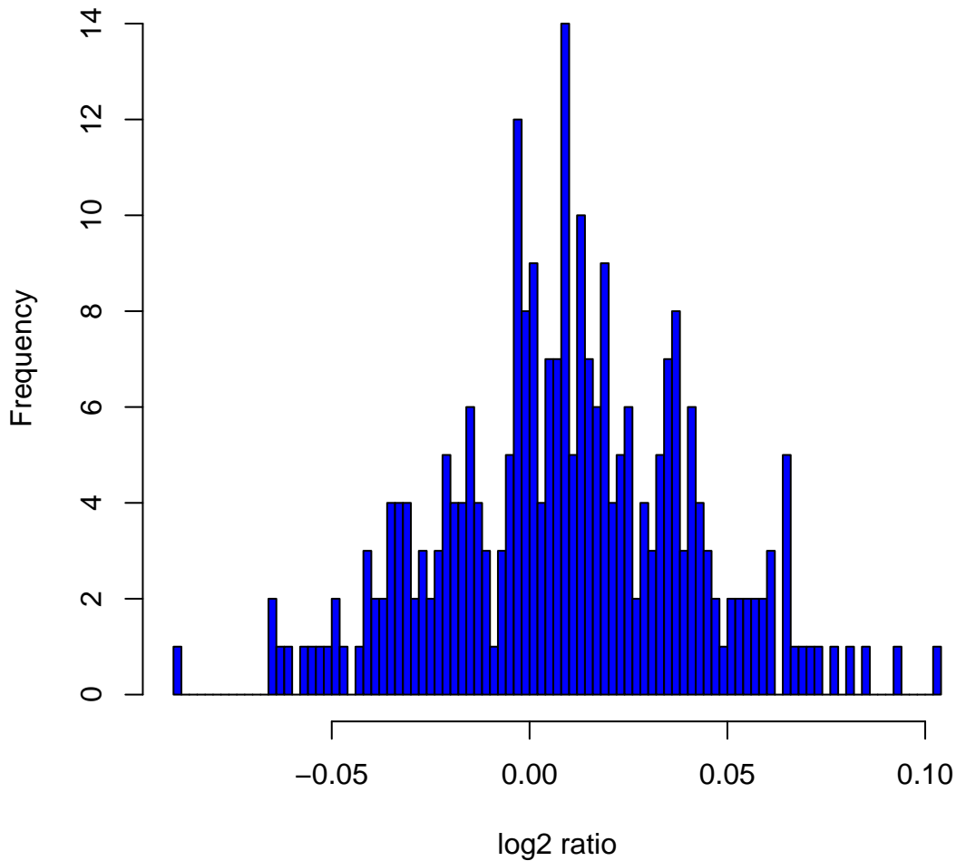
Histogram of log 2 ratios in 270 HapMap samples at clone Chr2tp-4A3
