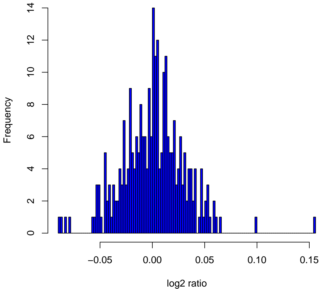
Histogram of log 2 ratios in 270 HapMap samples at clone Chr2tp-4B3
