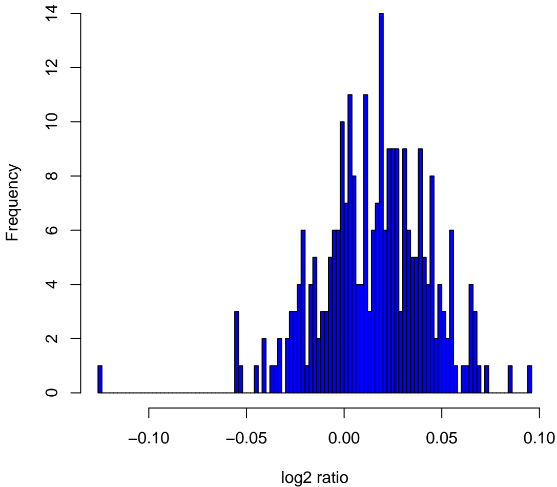
Histogram of log 2 ratios in 270 HapMap samples at clone Chr2tp-4B5
