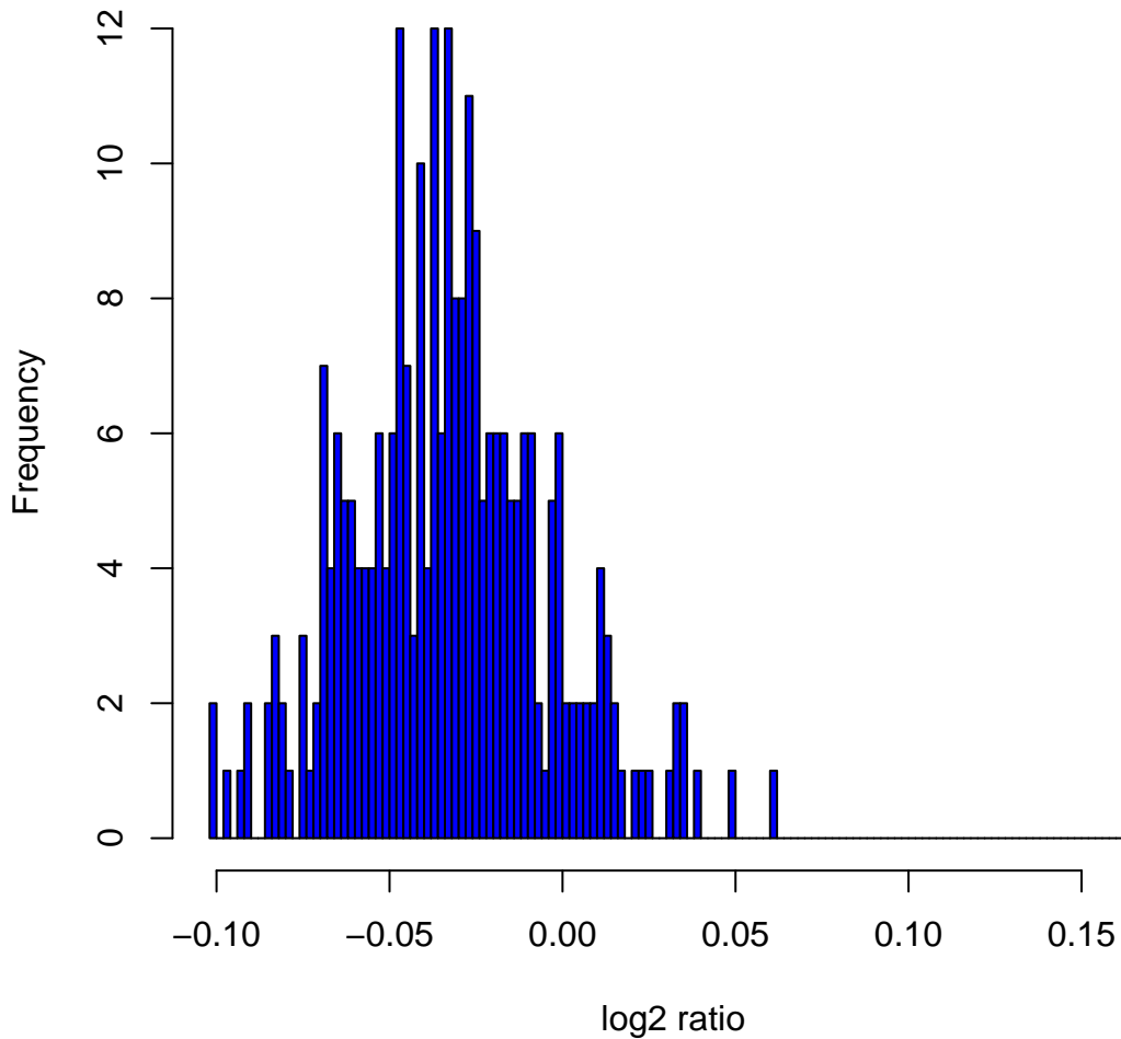
Histogram of log 2 ratios in 270 HapMap samples at clone Chr2tp-4C11
