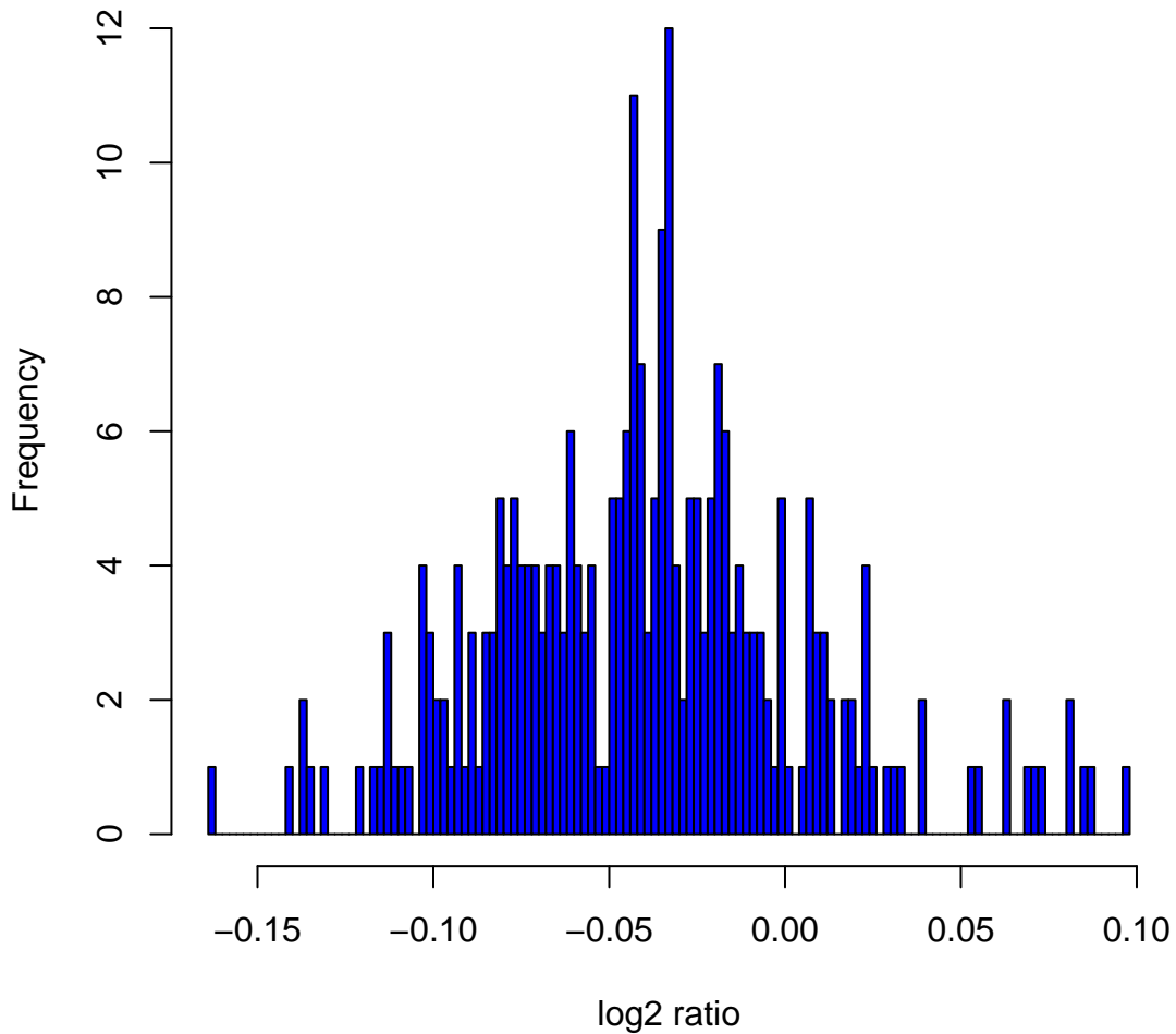
Histogram of log 2 ratios in 270 HapMap samples at clone Chr2tp-4C2
