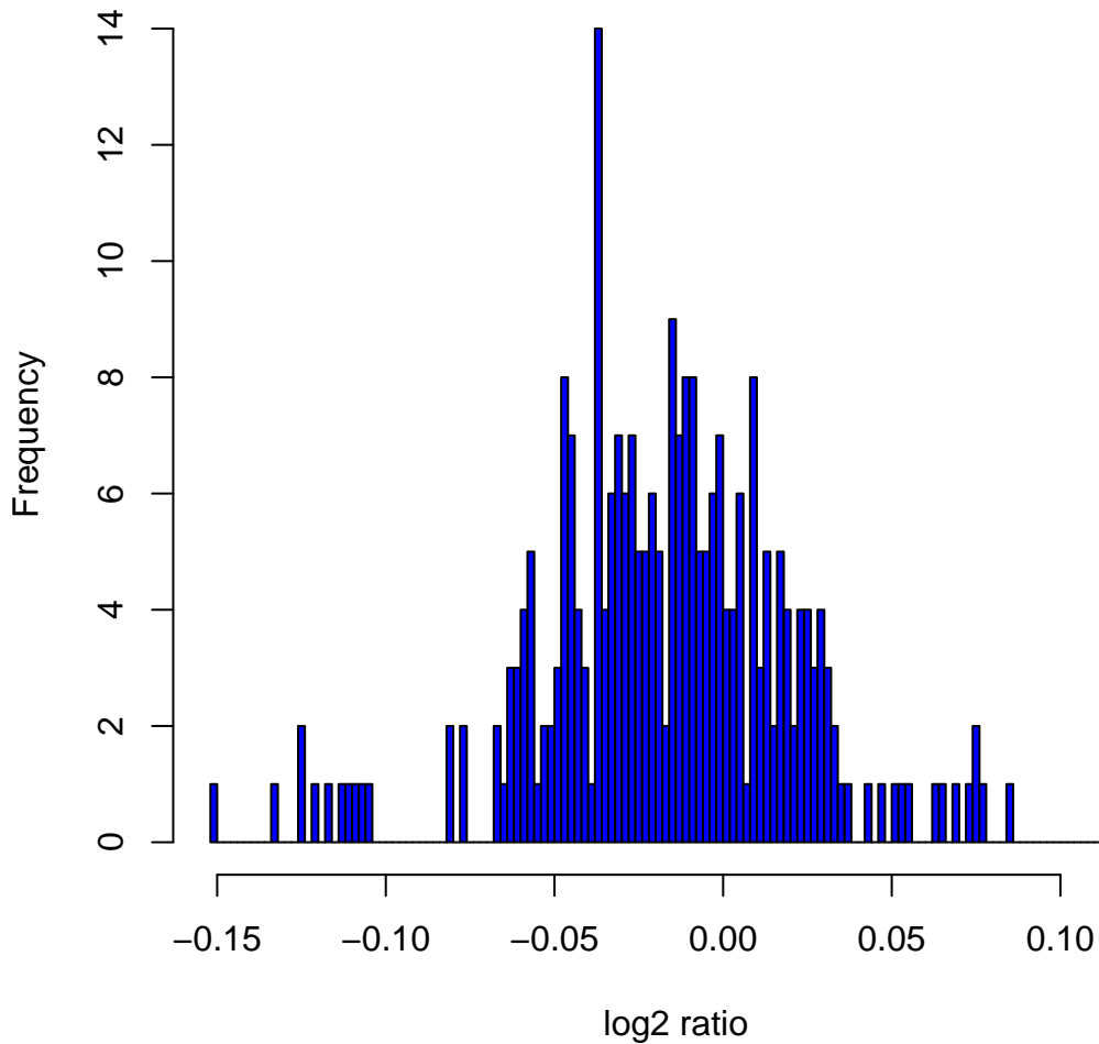
Histogram of log 2 ratios in 270 HapMap samples at clone Chr2tp-4E1
