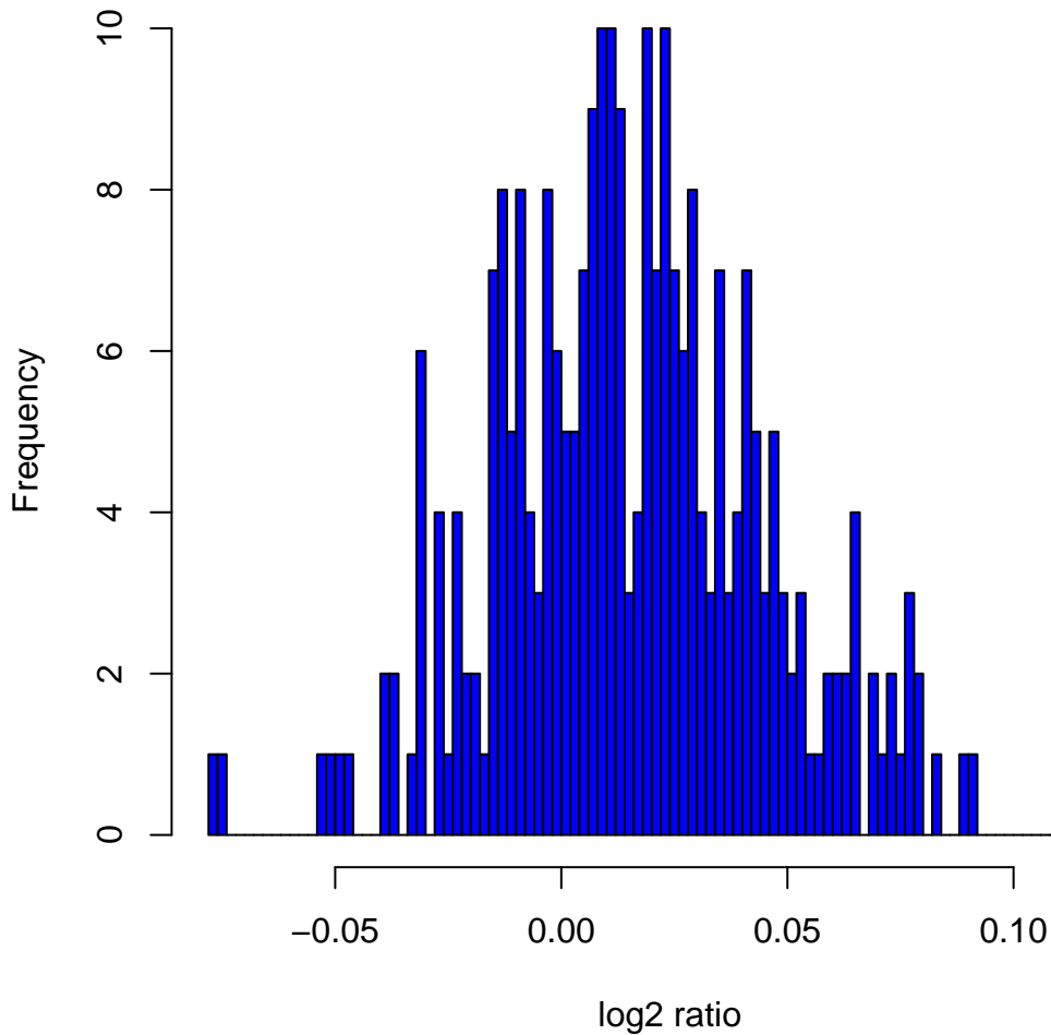
Histogram of \log_2 ratios in 270 HapMap samples at clone Chr2tp-4E5
