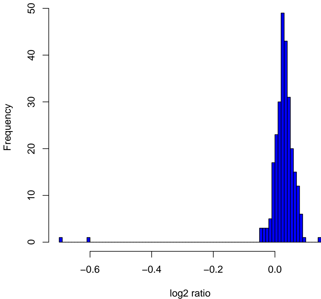
Histogram of log2ratios in 270 HapMap samples at clone Chr2tp-4F2
