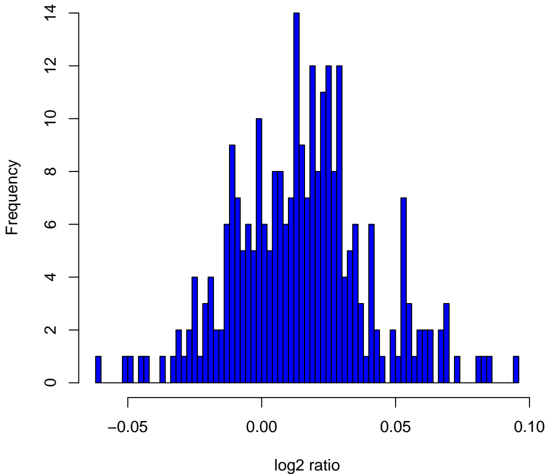
Histogram of log 2 ratios in 270 HapMap samples at clone Chr2tp-4G1
