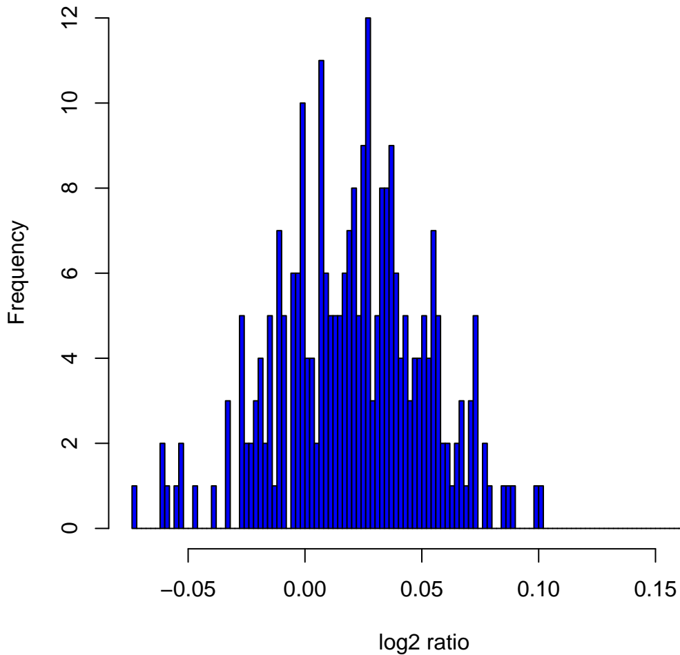
Histogram of \log_2 ratios in 270 HapMap samples at clone Chr2tp-4G3
