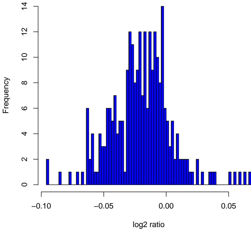
Histogram of log 2 ratios in 270 HapMap samples at clone Chr2tp-4G8
