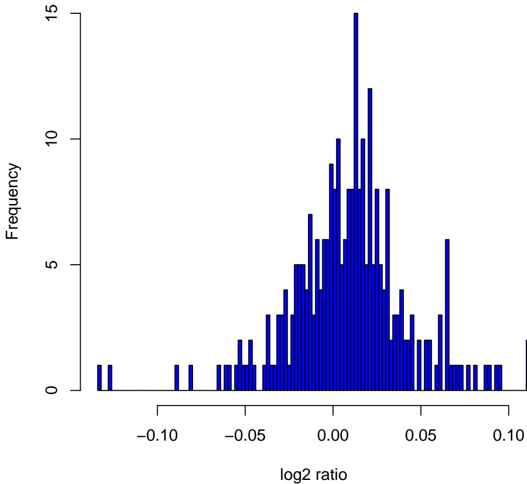
Histogram of log 2 ratios in 270 HapMap samples at clone Chr2tp-4H3
